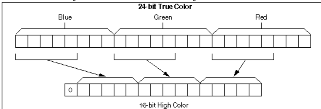
Figure 1. 24-bit True Color to 16-bit High Color Conversion
