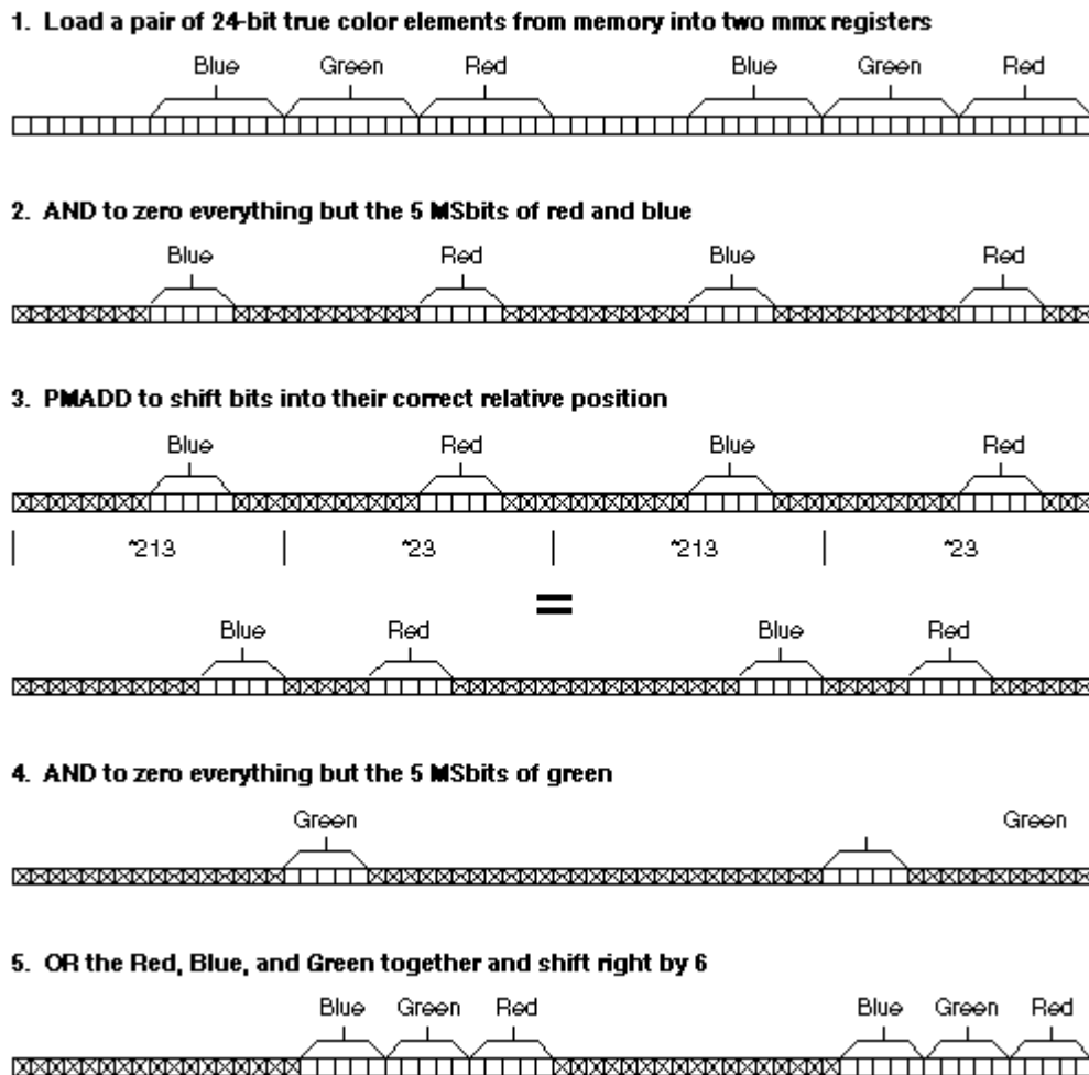
Figure 2. PMADD Basic Algorithm
