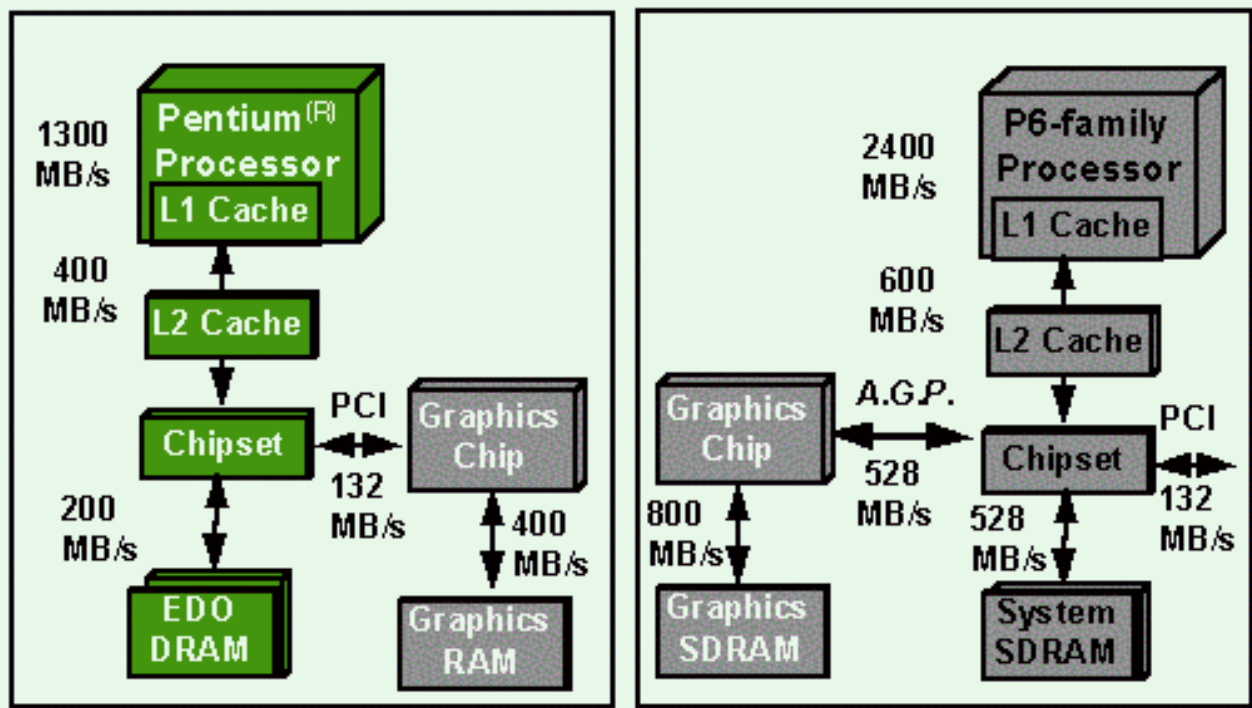
Figure 4: Peak Hardware Bandwidths for Two Typical Systems
