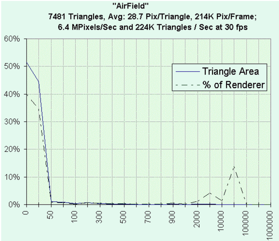
Figure 6: Polygon Size Distribution for a Sample 3D Flight Simulator Scene
