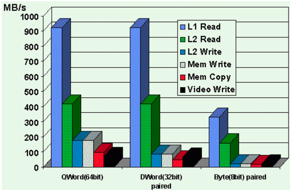
Figure 5: Measured Memory and Graphics Bandwidth for Pentium(R) Processor 166MHz 82430HX systems for various types of access
