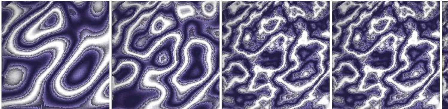
Figure 10.1: One octave
