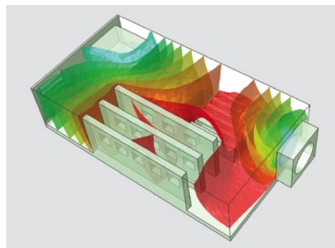
The native CFD capability in Abaqus 6.10 enables full system structural and thermal analysis in conjunction with natural/forced convection cooling, which can be used to study thermal performance of electronic products. This model shows temperature isosurfaces on an electronic circuit board model.
