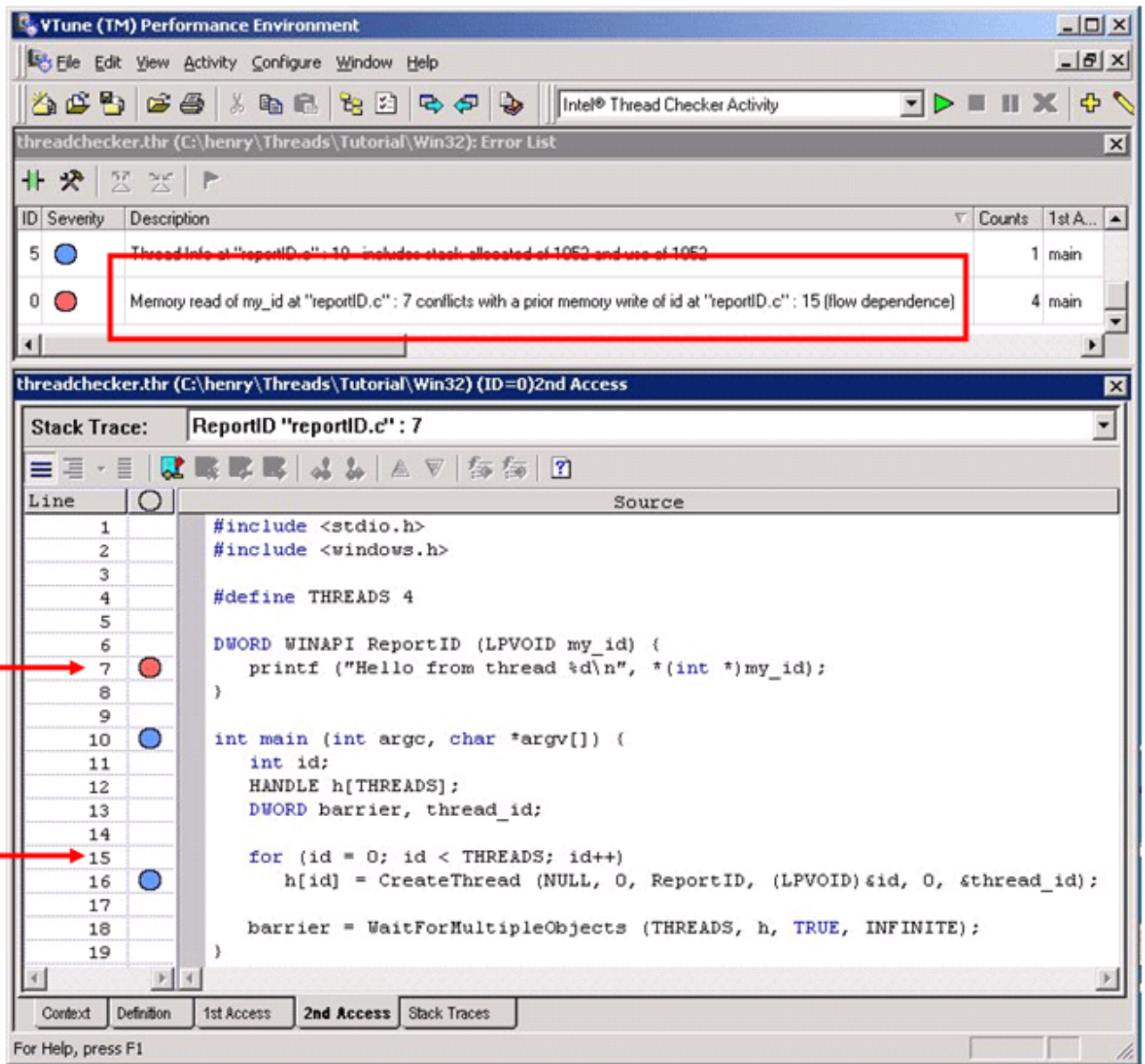
Figure 2: The Intel Thread Checker
