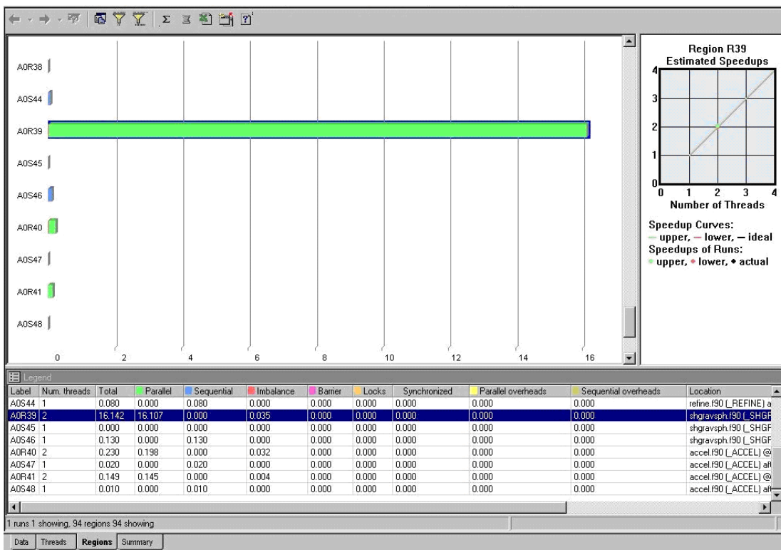
Figure 4: Regions View and Legend in Thread Profiler
