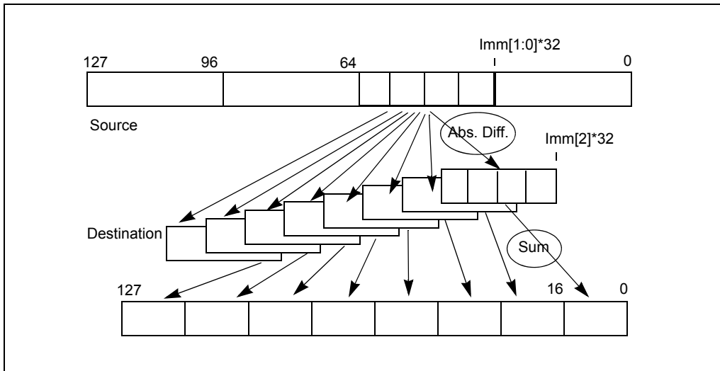
Figure 2-1. MPSADBW Operation
